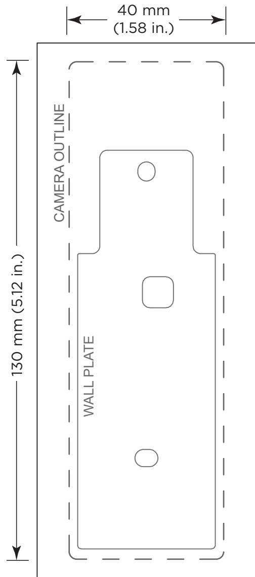
C4-VDB-W (Wi-Fi) template
